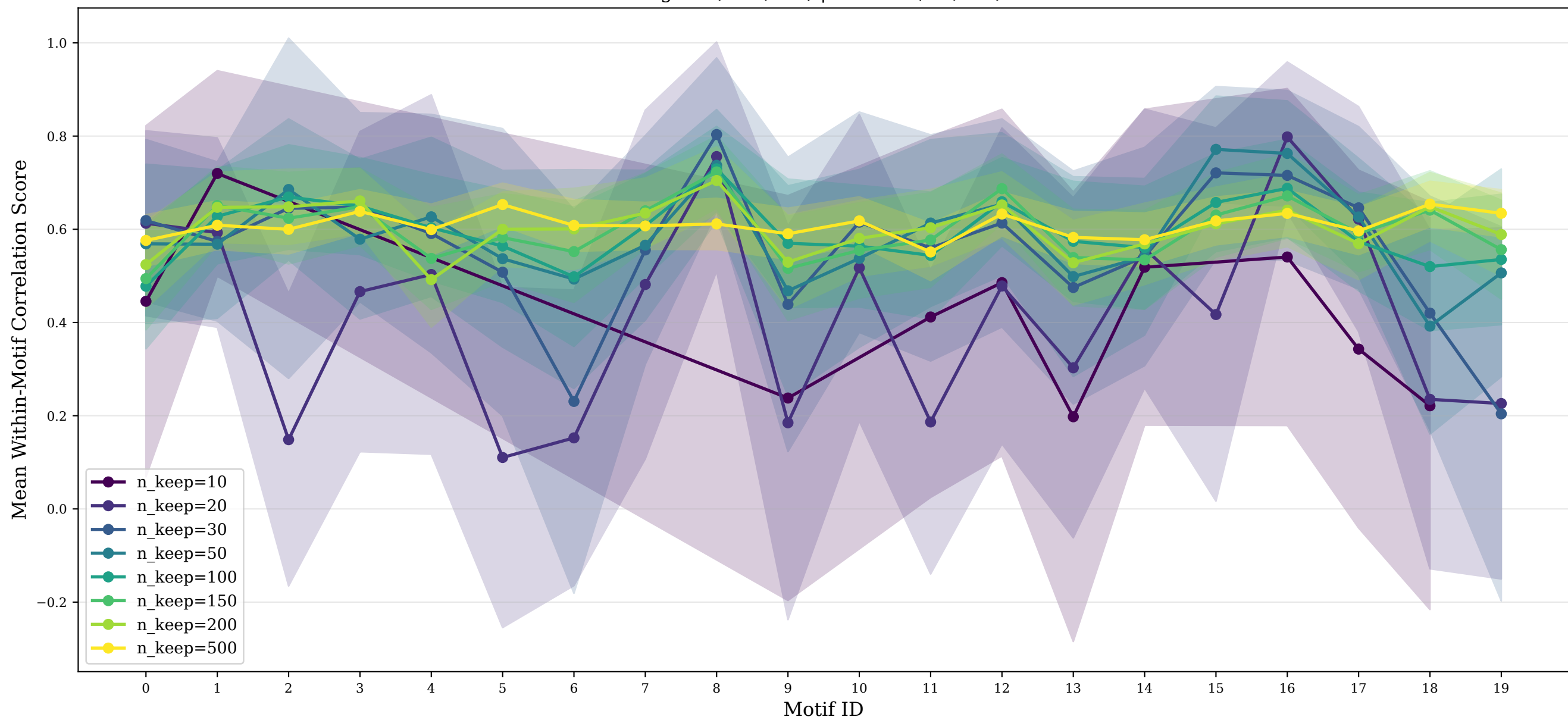
Correlation Score per Motif at Different Downsampling Levels (min_length=5) sigma: (0.02, 0.4) | volume: (0.1, 0.2)
